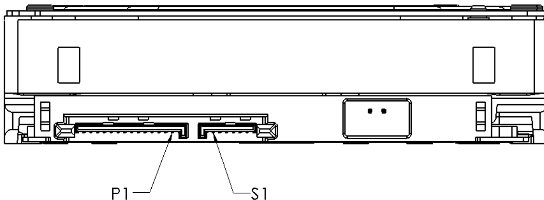
Figure 2 Connector Location
