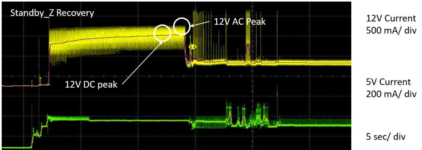
Figure 9 Standby_Z Recovery Current Waveform
