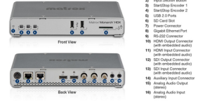
MATROX MONARCH HDX CONNECTIONS
