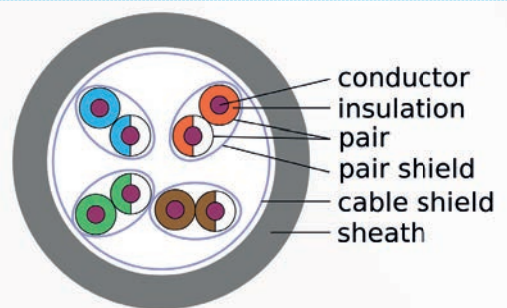
S-STP cable profile
