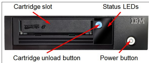
Figure 4. Front view of the TS2260
